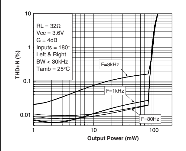
Figure 25. THD+N vs. output power
